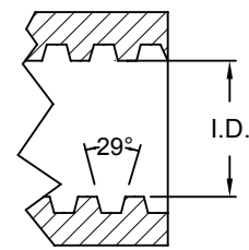
female thread
