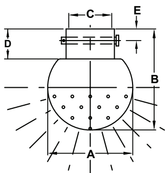
180° Bottom Pattern
